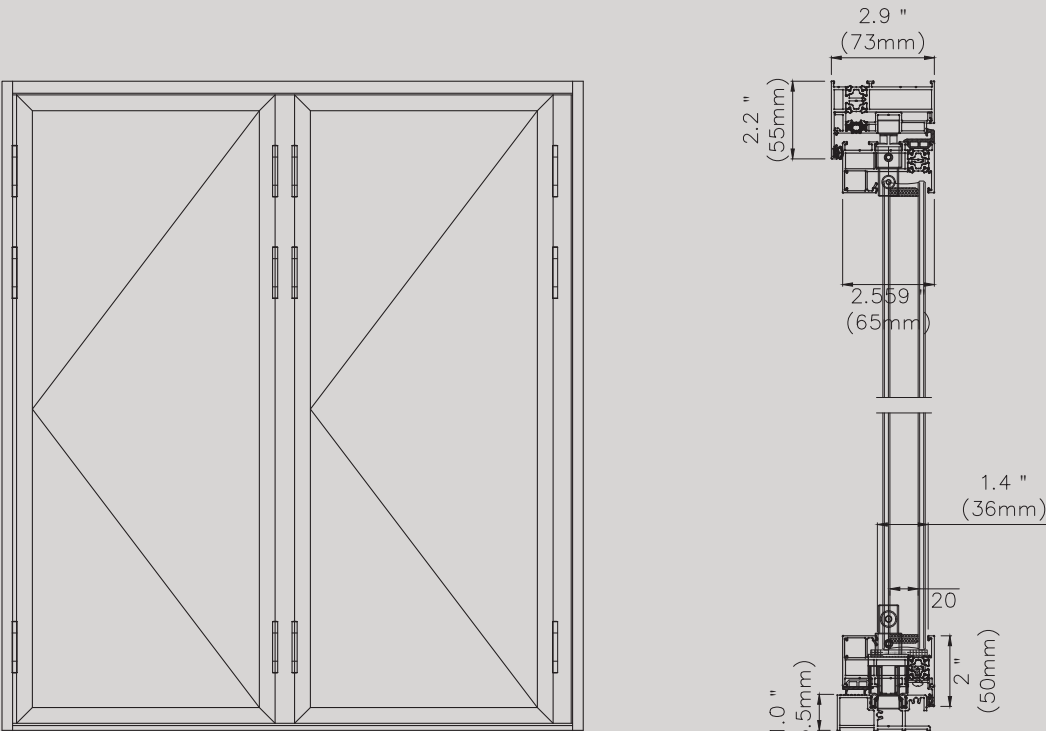
Outer folding low rail up and down positioning structure
